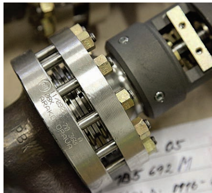
Detail ventilu
